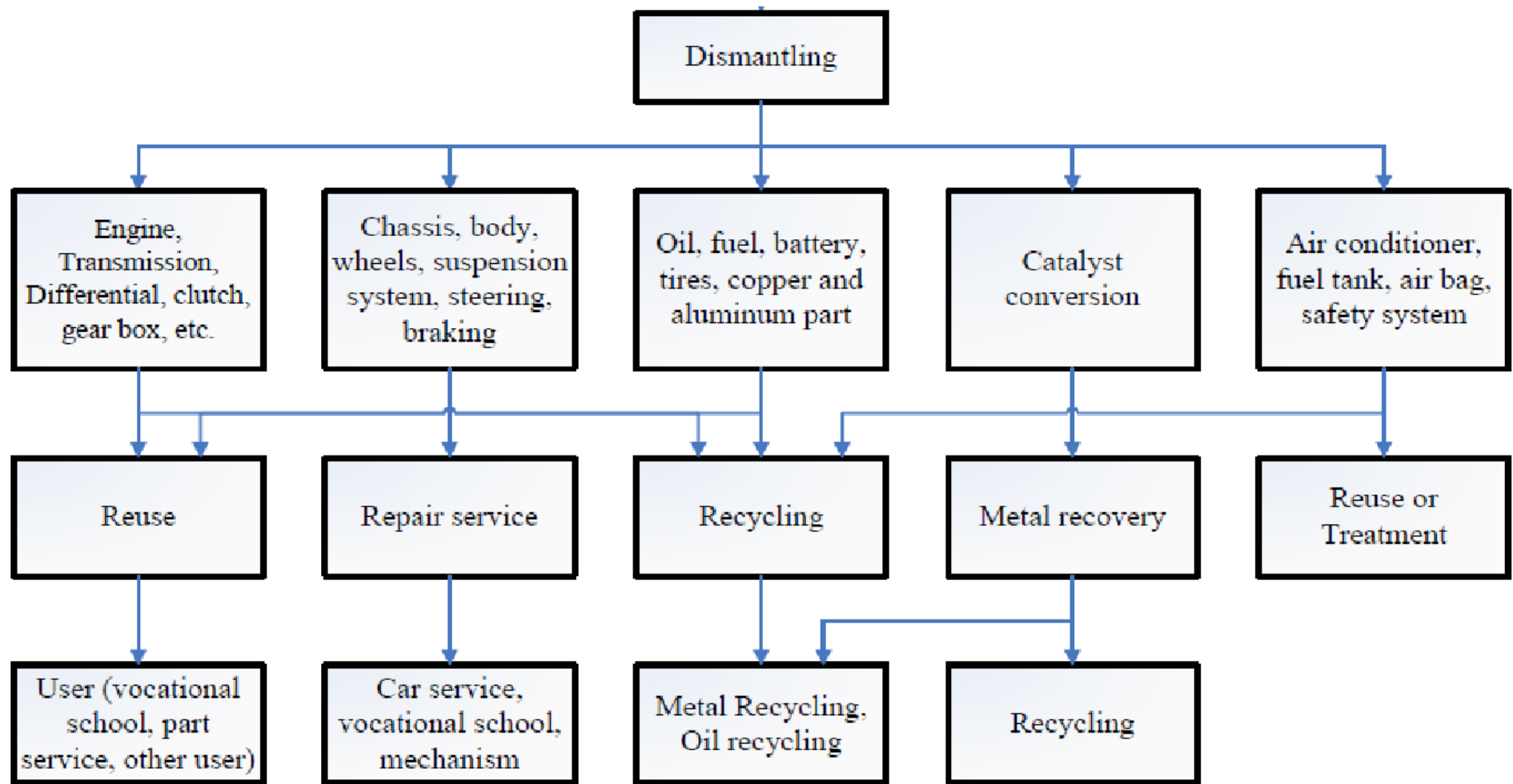
Figure 2.34. Common Flow of ELV in Dismantling Centres in Viet Nam
