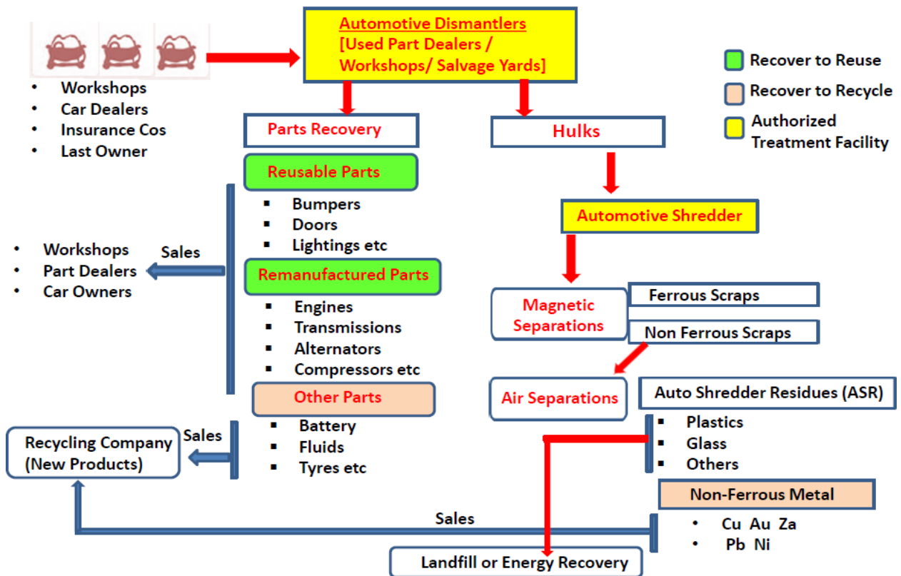
Figure 2.13. End-of-life Vehicle Recycling Process, Malaysia
